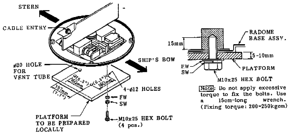
Fig.5 Installing the Scanner Unit
