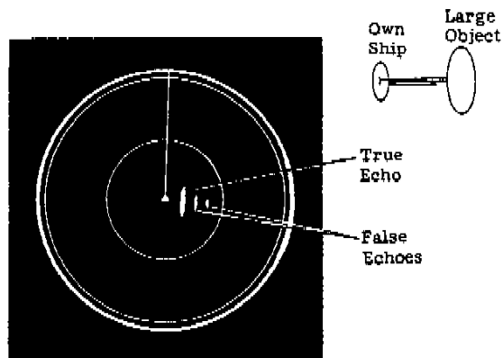
Fig.32 Multiple Echoes
