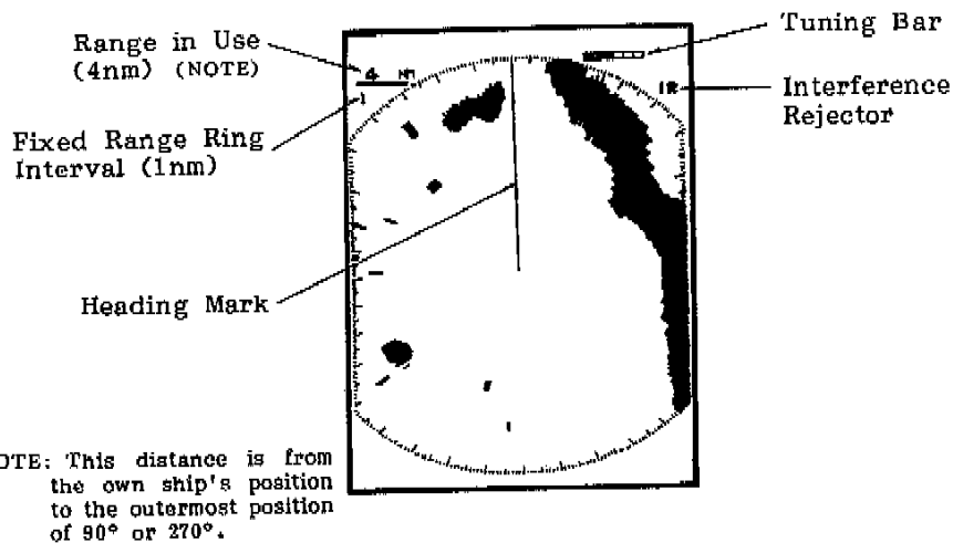
Fig.20 Location of Display Screen Indicators
