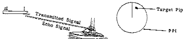
Fig.1 How Radar Works
