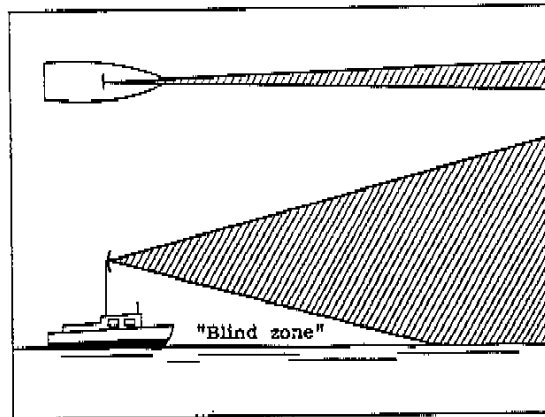
Fig.29 Effects of a Scanner Mounted too High off the Water
