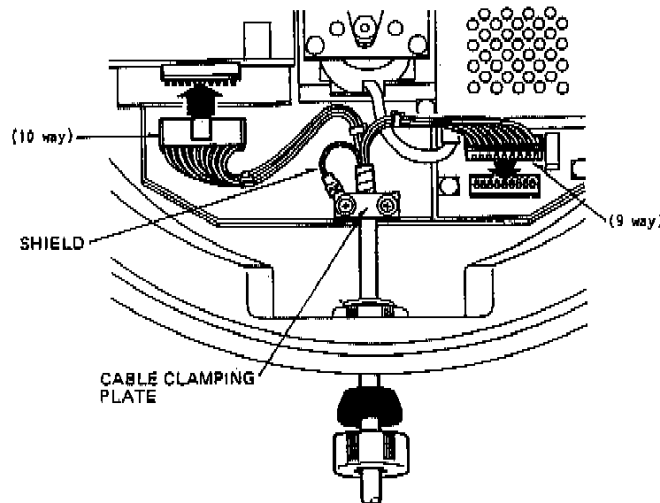
Fig.7 Cable Connection and Grounding
