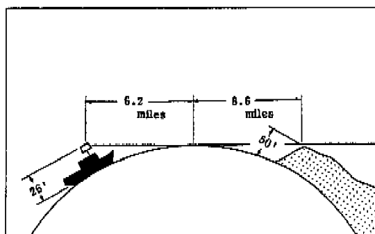
Fig.30 Radar Horizon
