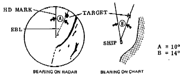
Fig.12 Relative Bearing Alignment
