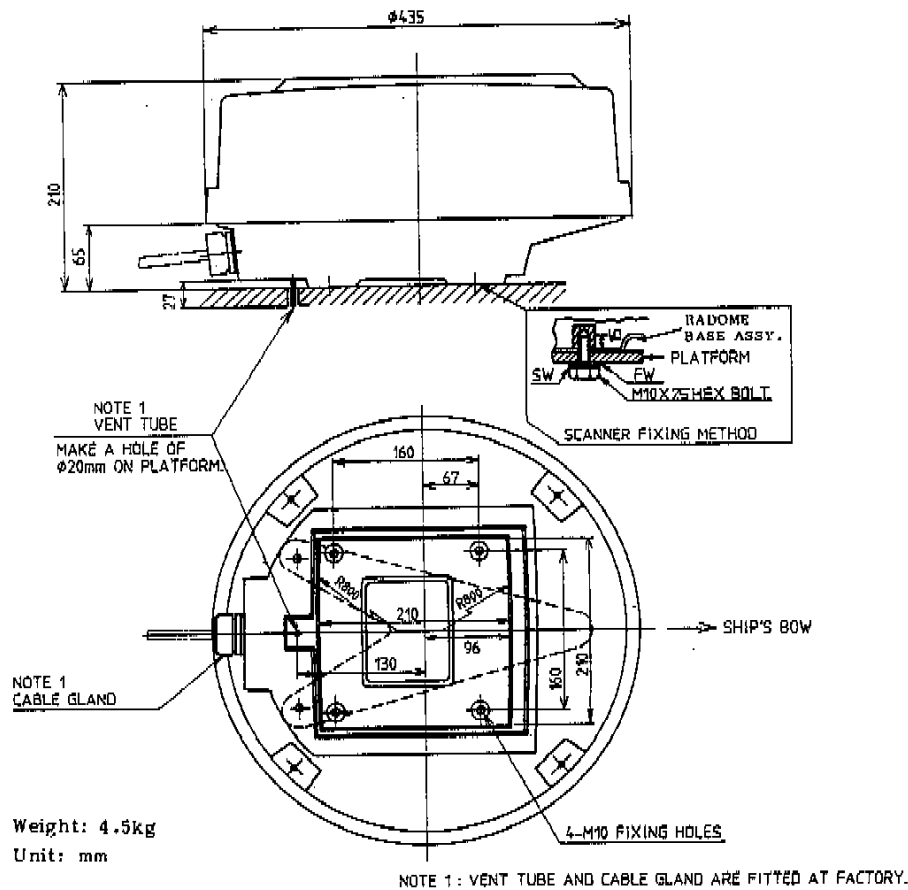
Fig.6 Scanner Unit Outline Drawing
