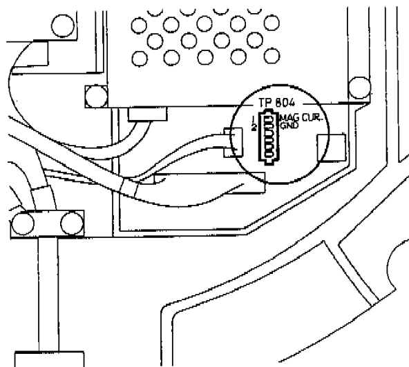
Fig.43 Measuring the Magnetron Current
