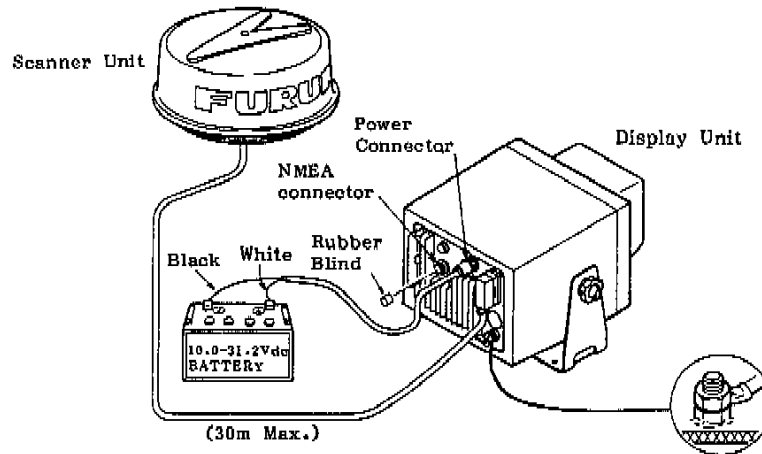
Fig.11 Detailed Wiring Diagram
