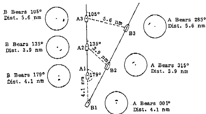
Fig.40 Relative Motion vs. True Motion
