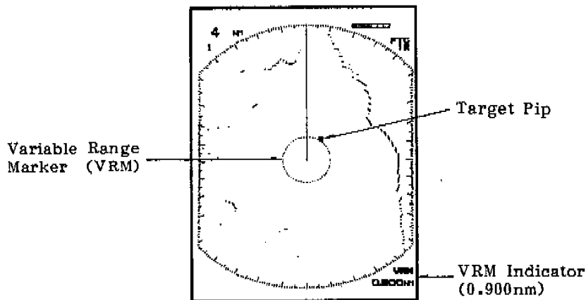
Fig.23 Range Measurement with the VRM Control
