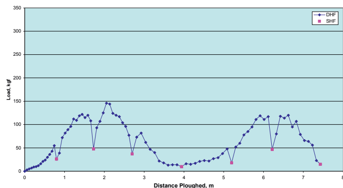
FIGURE 3. Plot of DHF and SHF against distance ploughed for 6.7kg CQR anchor. The anchor was initially laid on its side on the sand surface. Speed of ploughing about 2cm/sec. Reference UHC of SPADE = 135kgf
