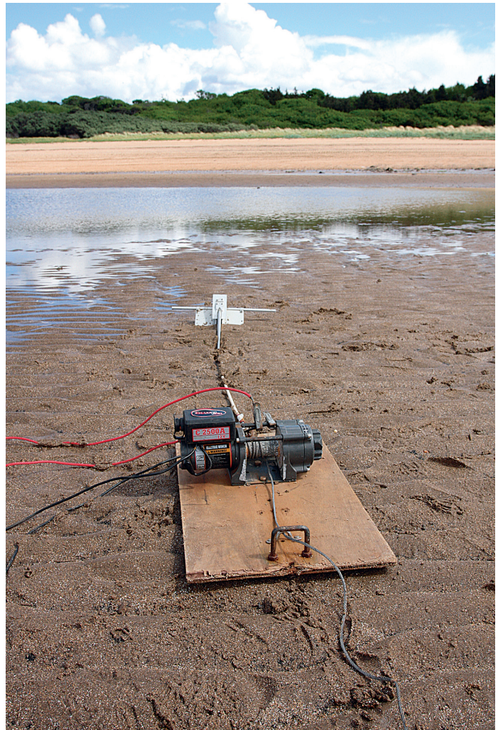
The load is shared between three anchors firmly embedded in the sand at the end of the purchase and the winch assembly (above)
