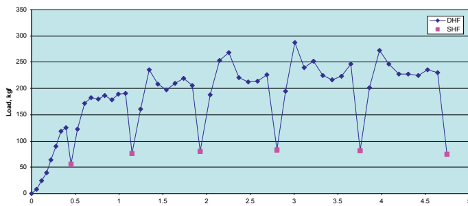
FIGURE 2A. Plot of DHF and SHF against distance ploughed for 16.1kg Bruce anchor. Speed of ploughing 3cm/sec. Reference UHC of SPADE = 120kgf
