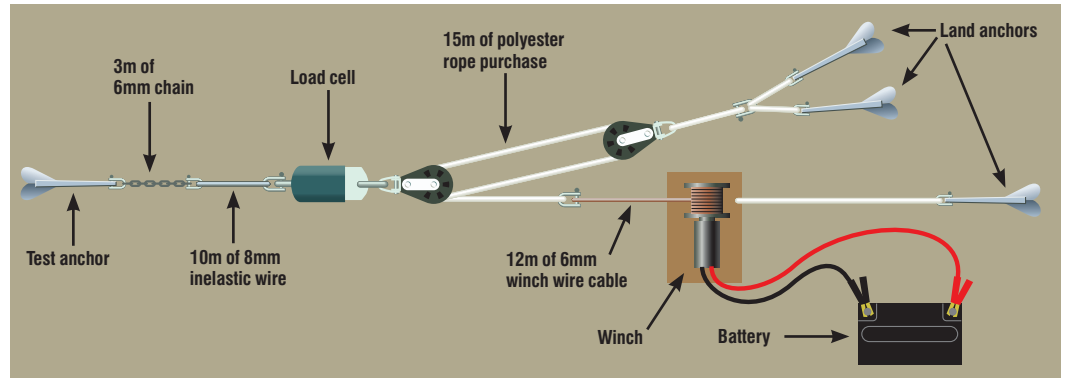
Diagram of pulling system used to determine SHF and DHF values
