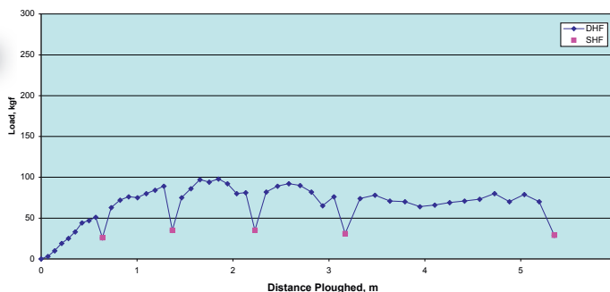
FIGURE 2. Plot of DHF and SHF against distance ploughed for 5.8kg Bruce anchor. Speed of ploughing about 2-3cm/sec. Reference UHC of SPADE = 113kgf
