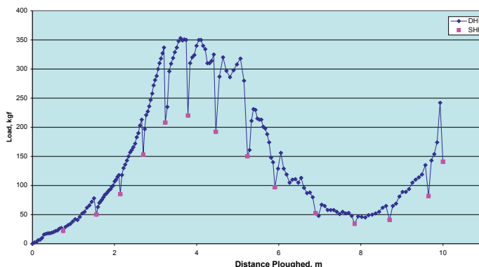
FIGURE 3A. Plot of DHF and SHF against distance ploughed for 21.5kg CQR anchor. The anchor was initially laid on its side on the sand surface. Speed of ploughing about 1 cm/sec. Reference UHC of SPADE = 150kgf
