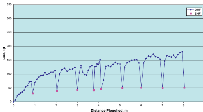
FIGURE 2B. Plot of DHF and SHF against distance ploughed for 4.9kg Atlantic (Bruce-type) anchor. Speed of ploughing about 2-3cm/sec. Reference UHC of SPADE = 135kgf
