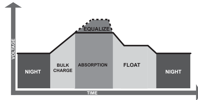
Figure 9. Algorithme de charges du SunSaver MPPT
