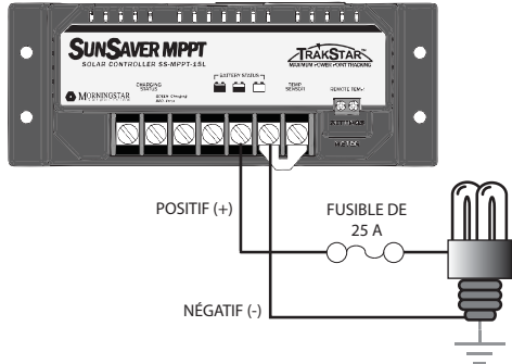
Figure 4. Câblage de charge
