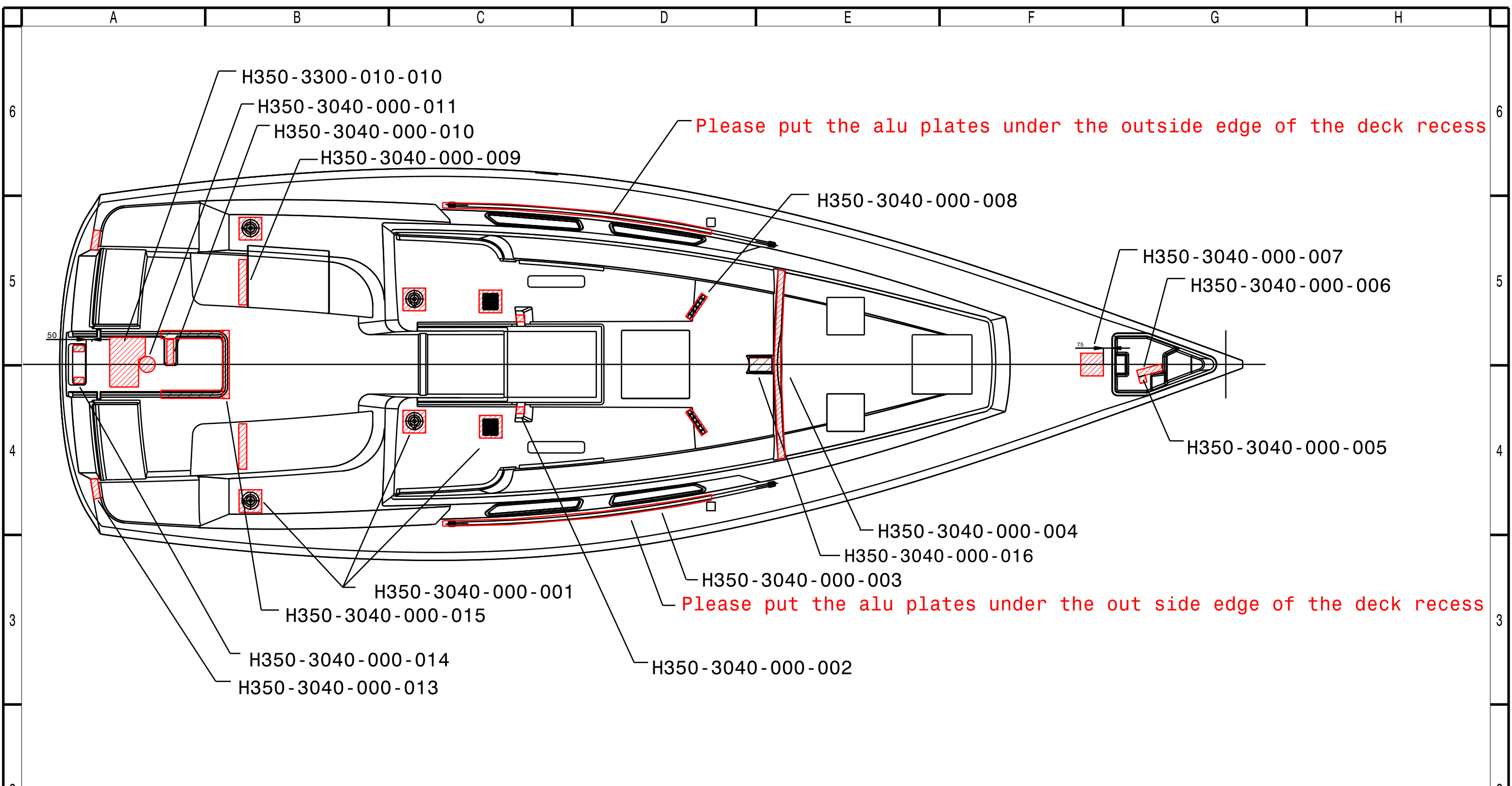
List of metal reinforcements.
