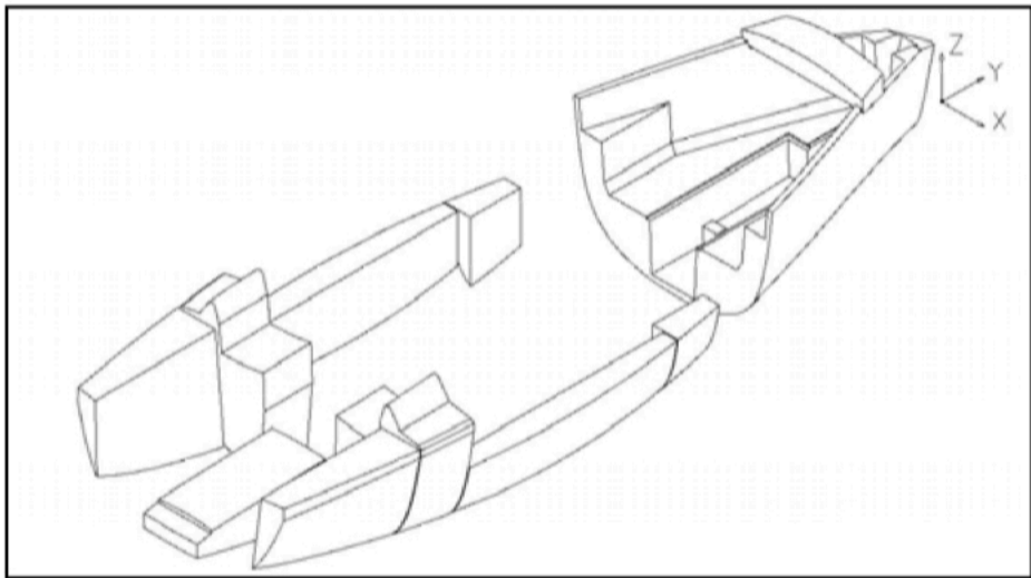
Volume of foam in ETAP 24i
