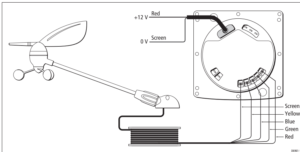
Figure 5: Test connections
